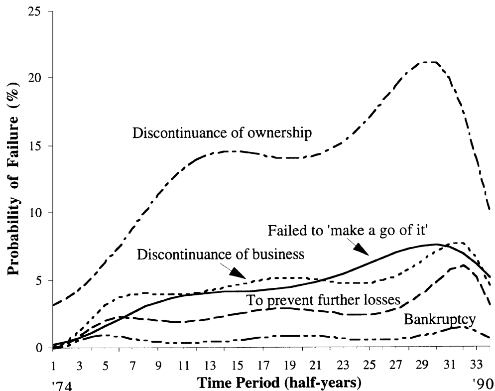
Figure 4. Probability of failure as a function of time period, for an average aged business.
