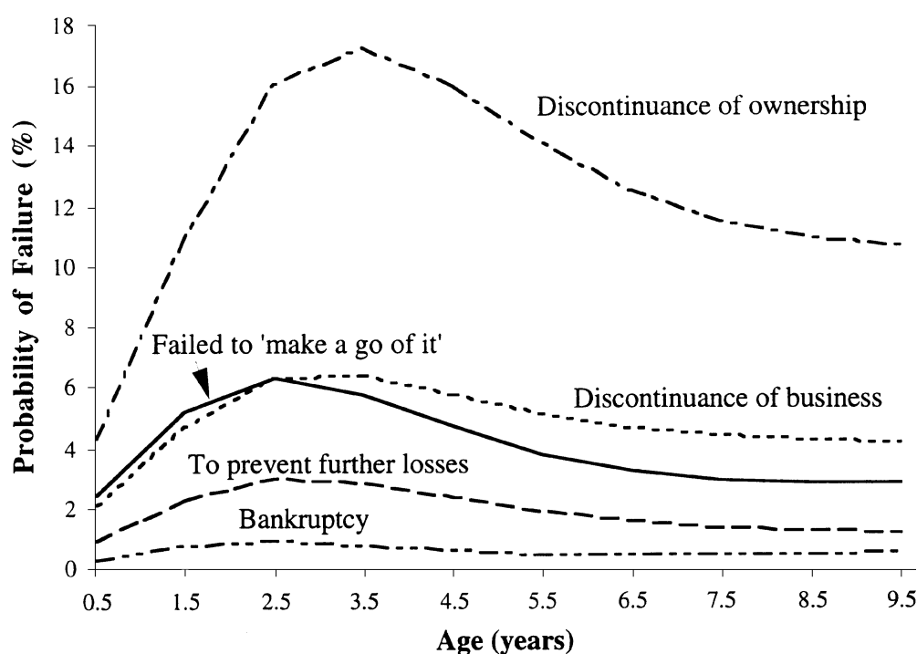
Figure 3. Probability of failure as a function of age, for an average time period.
