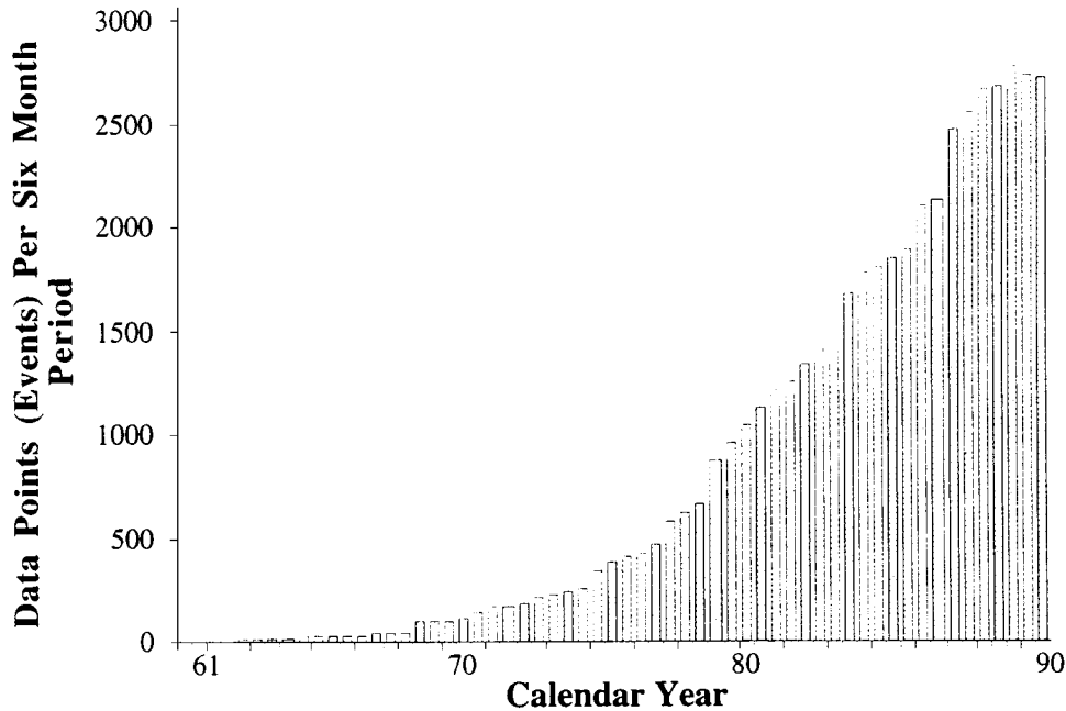
Figure 2. Data distribution across time where failure is defined as failed to "make a go of it".
